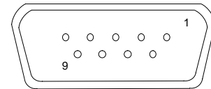
Figure 9-3. RS-232 Connector
